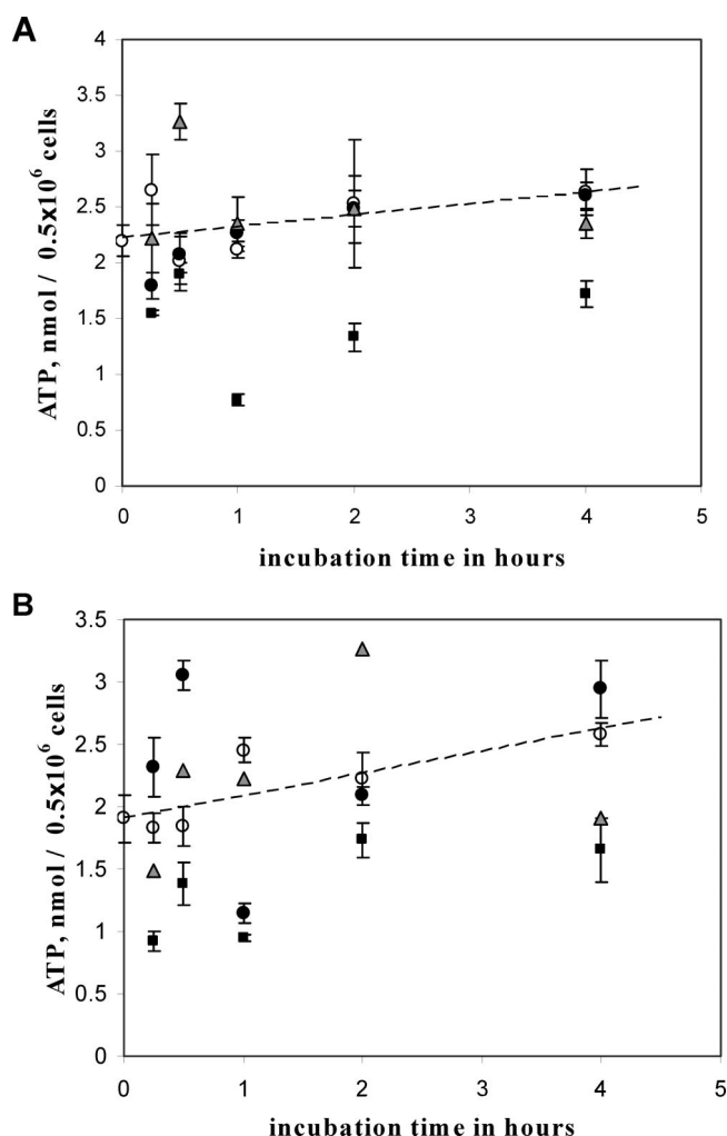
Figure 5. Effects of silica nanoparticles on cellular ATP. (A) Jurkat cells ( 0.5 \times 10^6 per mL) were incubated at 37 ^\circ\text{C} for indicated periods of time without additions (open circles) or with 50 \mu\text{g/mL} SBA-15 (closed circles), 50 \mu\text{g/mL} MCM-41 (triangles), or 10 mM NaCN (squares). Measured ATP concentrations are plotted vs incubation time; each is the average of three to five determinations, with the error bars giving standard deviations. Since the slope of the best-fit line for untreated cells (dashed) has slope \sim 0 , time-average ATP concentrations were calculated. (B) HL-60 cells ( 0.5 \times 10^6 per mL) were incubated at 37 ^\circ\text{C} for indicated periods of time without additions (open circles) or with 50 \mu\text{g/mL} SBA-15 (closed circles), 50 \mu\text{g/mL} MCM-41 (triangles), or 10 mM NaCN (squares). The best-fit line (dashed) for untreated cells has a very small slope, so average ATP levels were calculated as for Jurkat cells.
