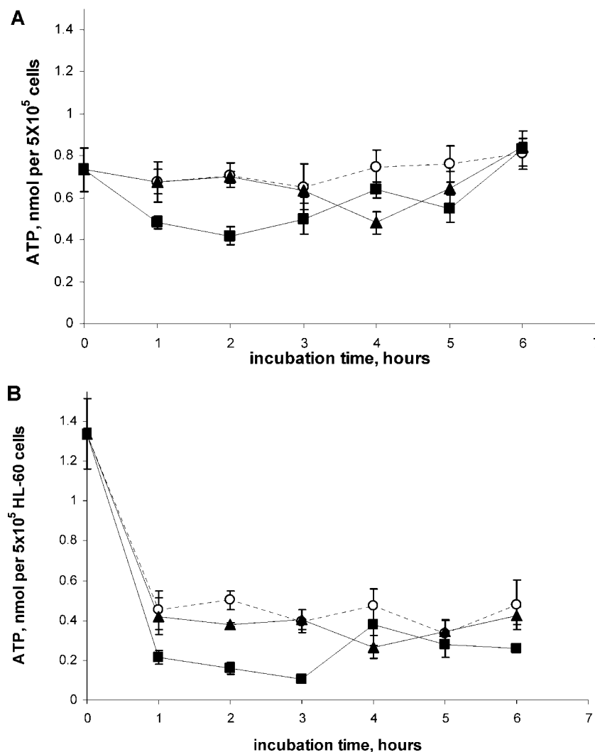
Figure 6. (A) HL-60 cells ( 0.5 \times 10^6 per mL) were incubated at 37 °C for indicated periods of time without or with 200 \mu g/mL SBA-15 or 200 \mu g/mL MCM-41. ATP levels were measured three to five times for each condition at t = 1 –6 h. Open circles, no addition; filled squares, 200 \mu g/mL SBA-15; filled triangles, 200 \mu g/mL MCM-41. (B) The experiment in panel A was repeated in the presence of 10 mM NaCN. Open circles, NaCN alone; closed squares, NaCN plus 200 \mu g/mL SBA-15; closed triangles, NaCN plus 200 \mu g/mL MCM-41. Standard deviations are indicated with error bars.
